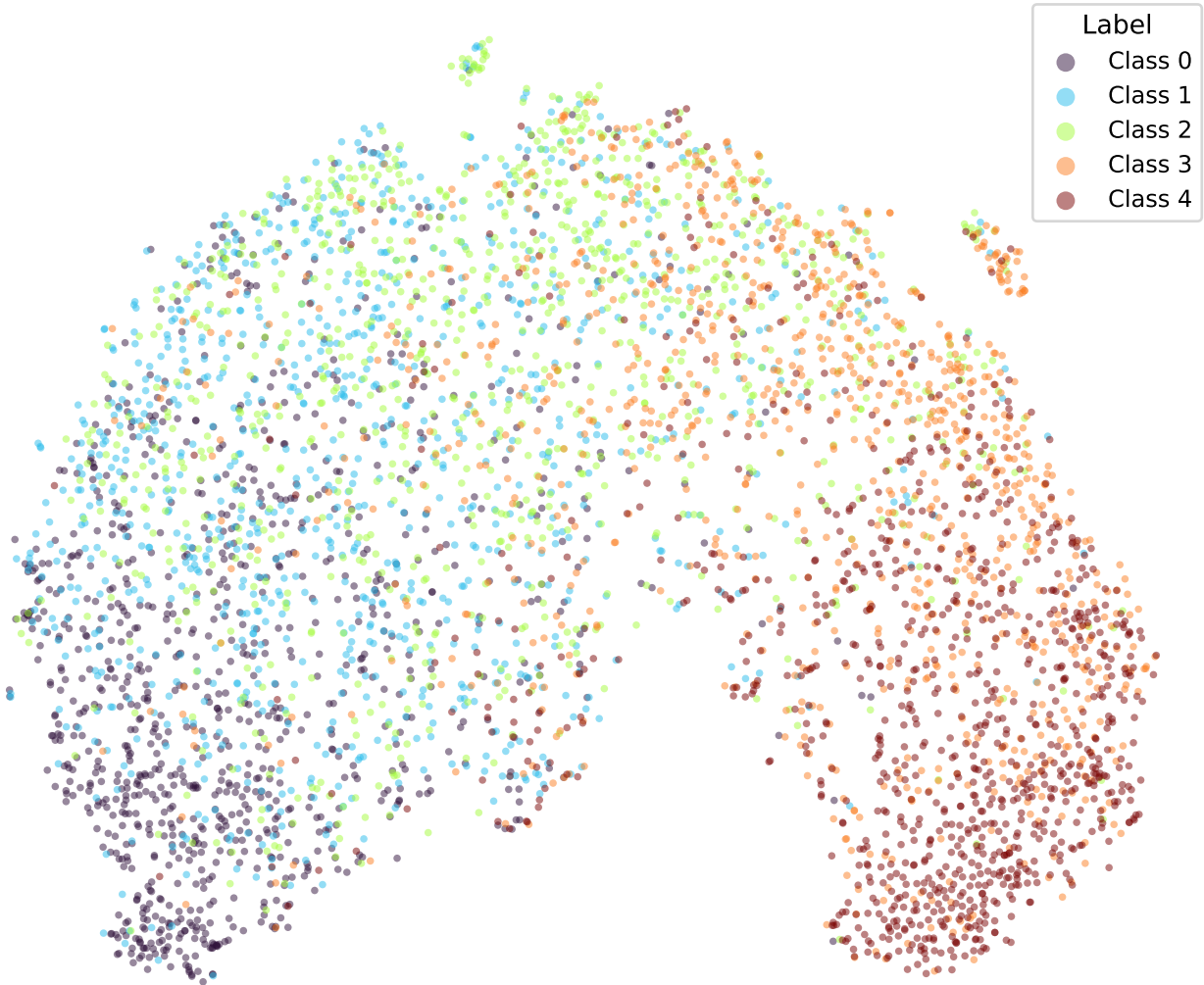
google/bert_uncased_L-2_H-128_A-2-amazon_reviews-CORN-1 (val)
