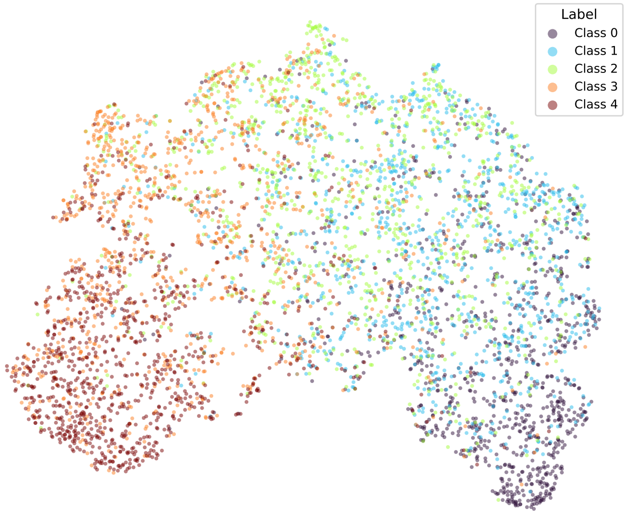
google/bert_uncased_L-2_H-128_A-2-amazon_reviews-CORN-2 (val)
