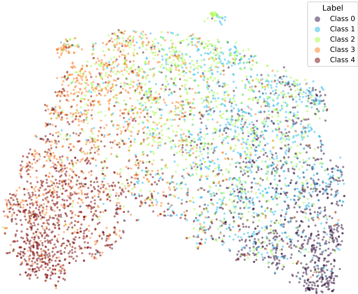
google/bert_uncased_L-2_H-128_A-2-amazon_reviews-CORN-2 (val)
