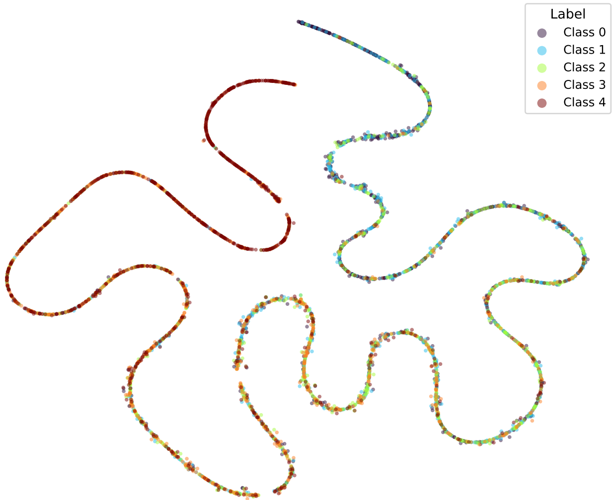
google/bert_uncased_L-2_H-128_A-2-amazon_reviews-CORN-3 (val)
