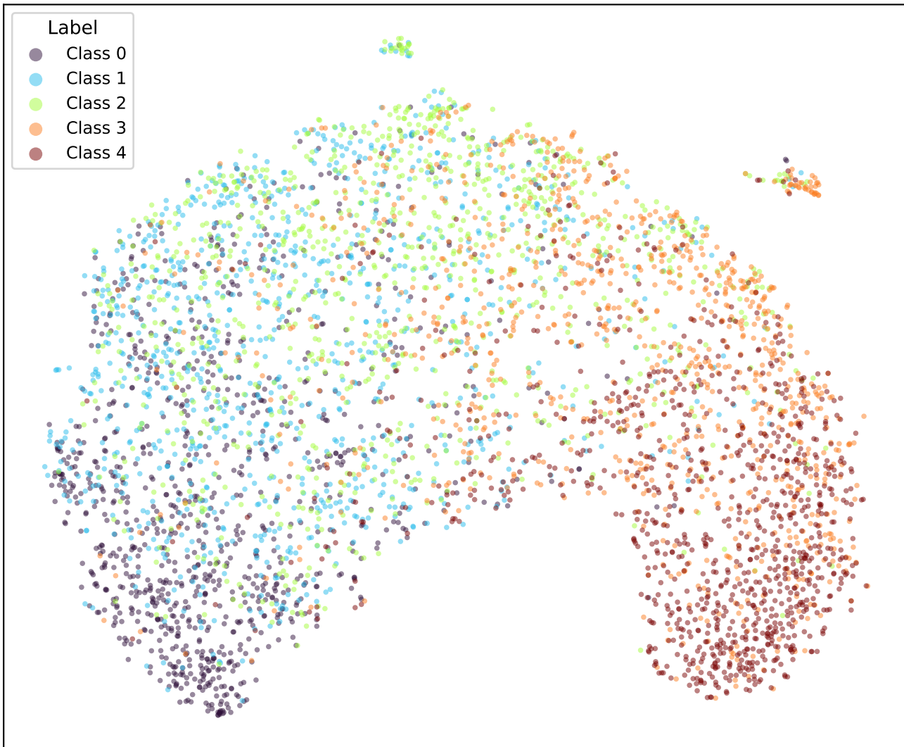
google/bert_uncased_L-2_H-128_A-2-amazon_reviews-CORN-3 (val)
