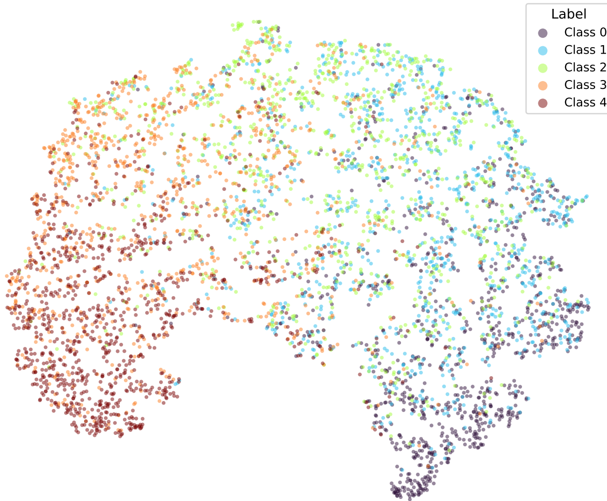
google/bert_uncased_L-2_H-128_A-2-amazon_reviews-CORN-4 (val)
