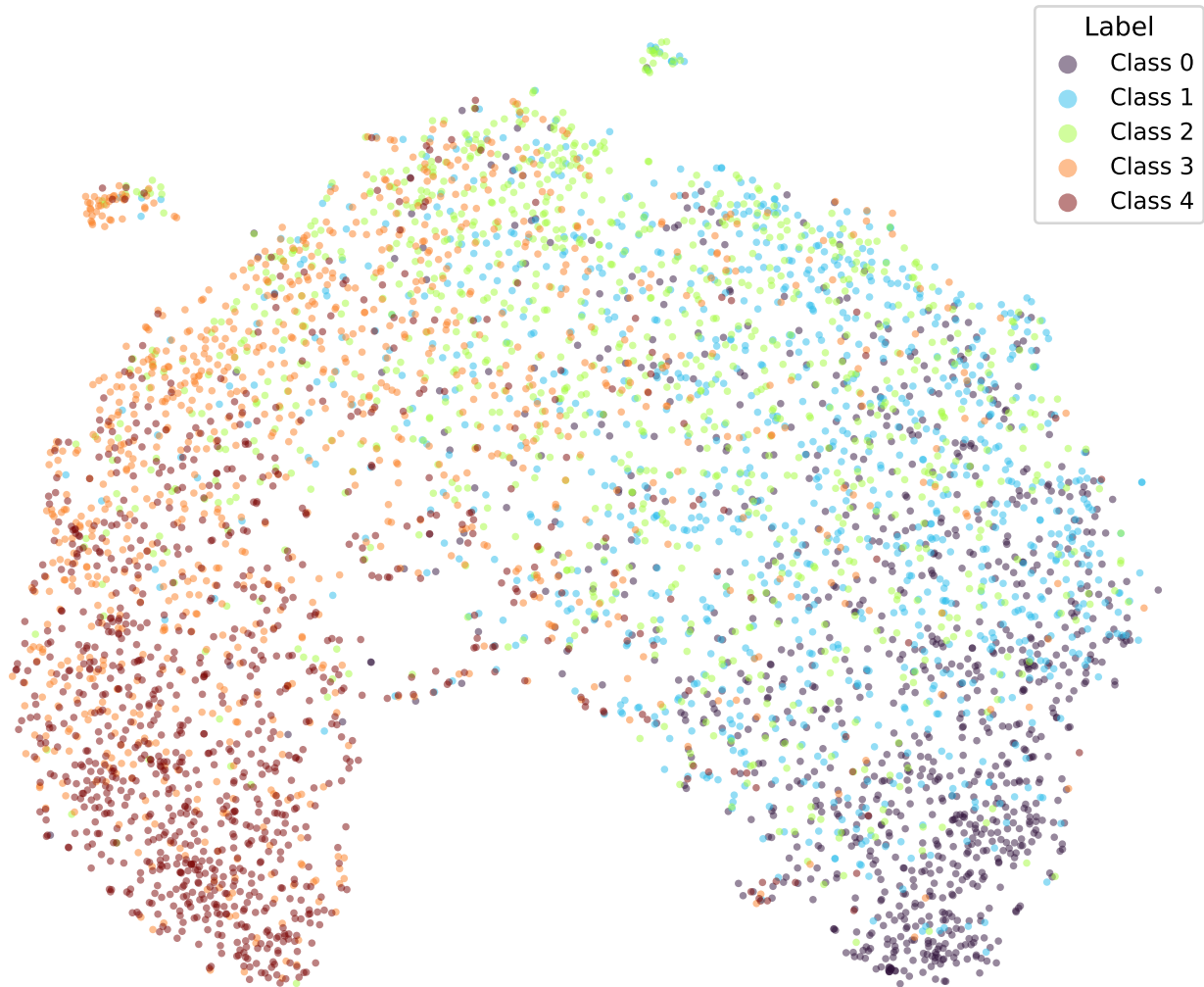
google/bert_uncased_L-2_H-128_A-2-amazon_reviews-CORN-4 (val)
