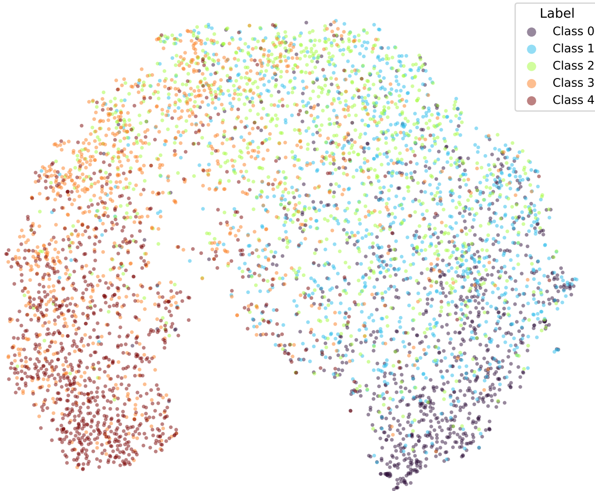
google/bert_uncased_L-2_H-128_A-2-amazon_reviews-CORN-5 (val)
