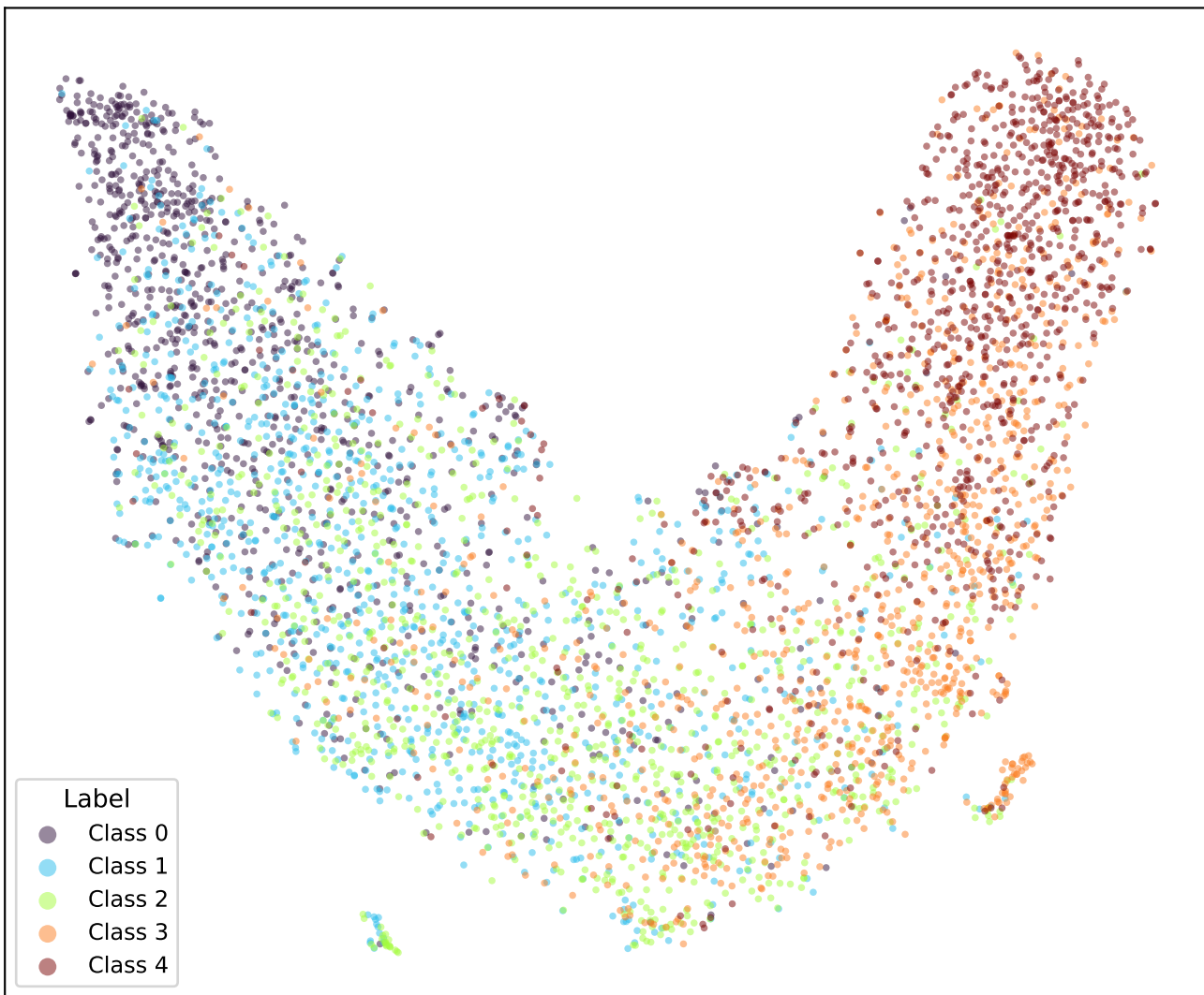
google/bert_uncased_L-2_H-128_A-2-amazon_reviews-EMD-TRIPa1-1 (val)
