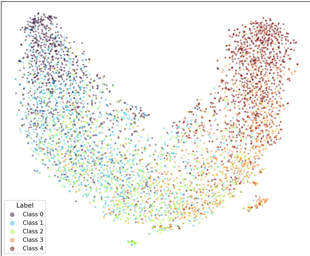
google/bert_uncased_L-2_H-128_A-2-amazon_reviews-EMD-TRIPa1-3 (val)
