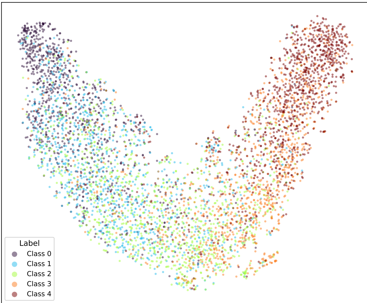
google/bert_uncased_L-2_H-128_A-2-amazon_reviews-EMD-TRIPa1-4 (val)
