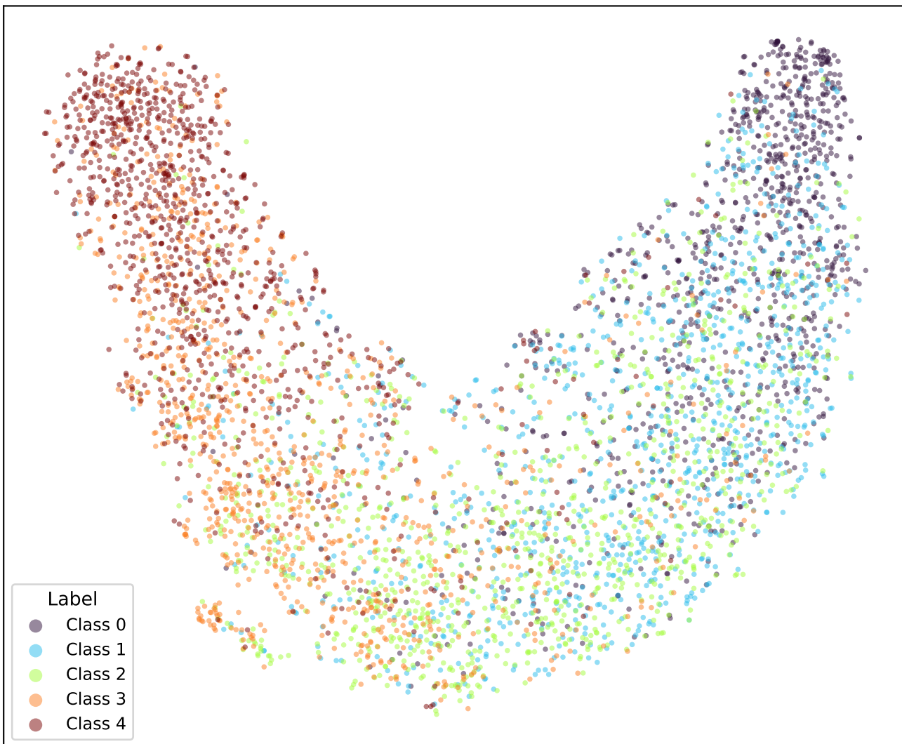
google/bert_uncased_L-2_H-128_A-2-amazon_reviews-EMD-TRIPa1-5 (val)
