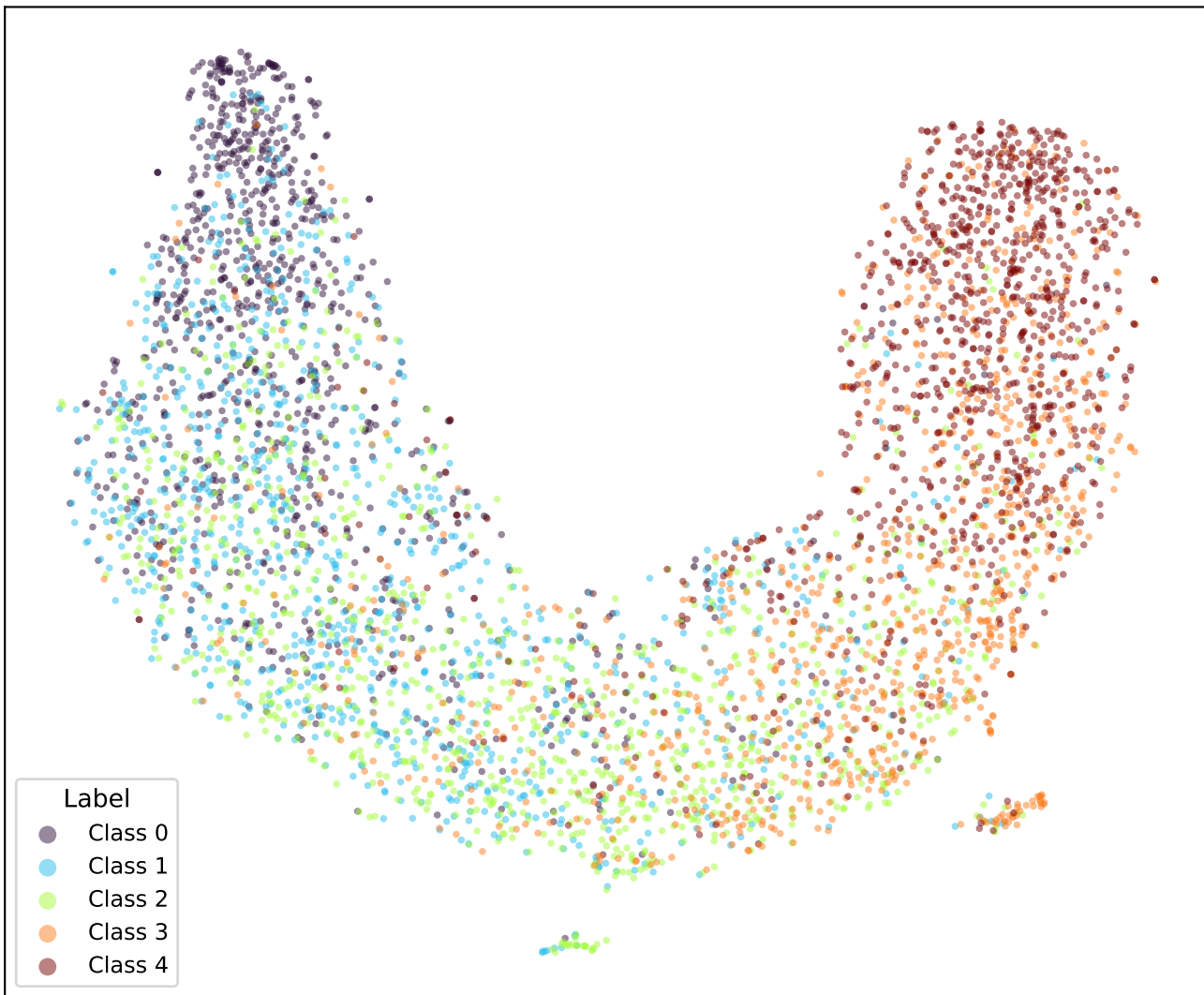
google/bert_uncased_L-2_H-128_A-2-amazon_reviews-OLL15-TRIPa1-3 (val)
