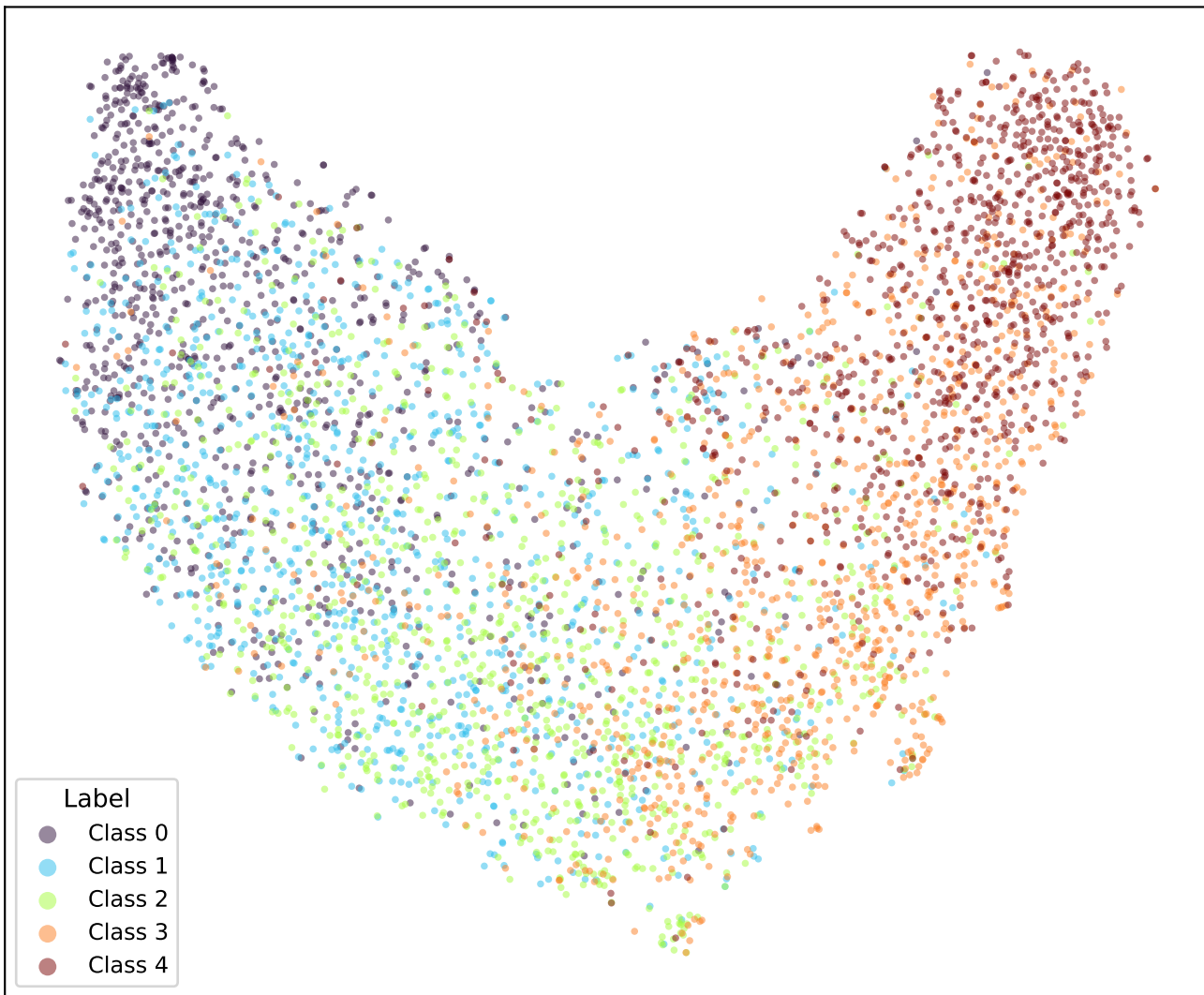
google/bert_uncased_L-2_H-128_A-2-amazon_reviews-SOFT2-TRIPa1-4 (val)
