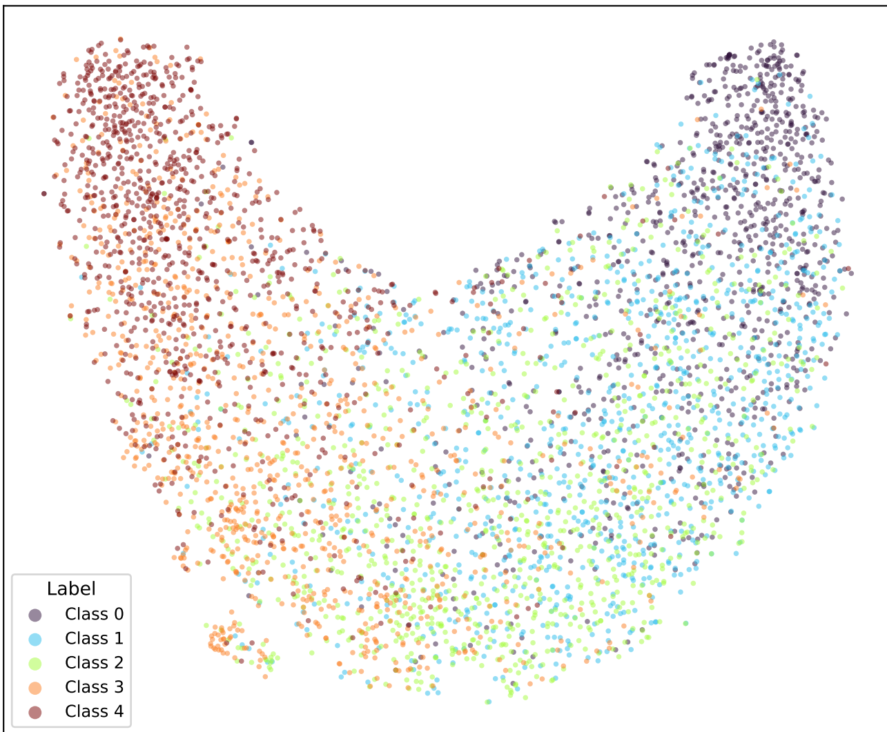
google/bert_uncased_L-2_H-128_A-2-amazon_reviews-SOFT2-TRIPa1-5 (val)
