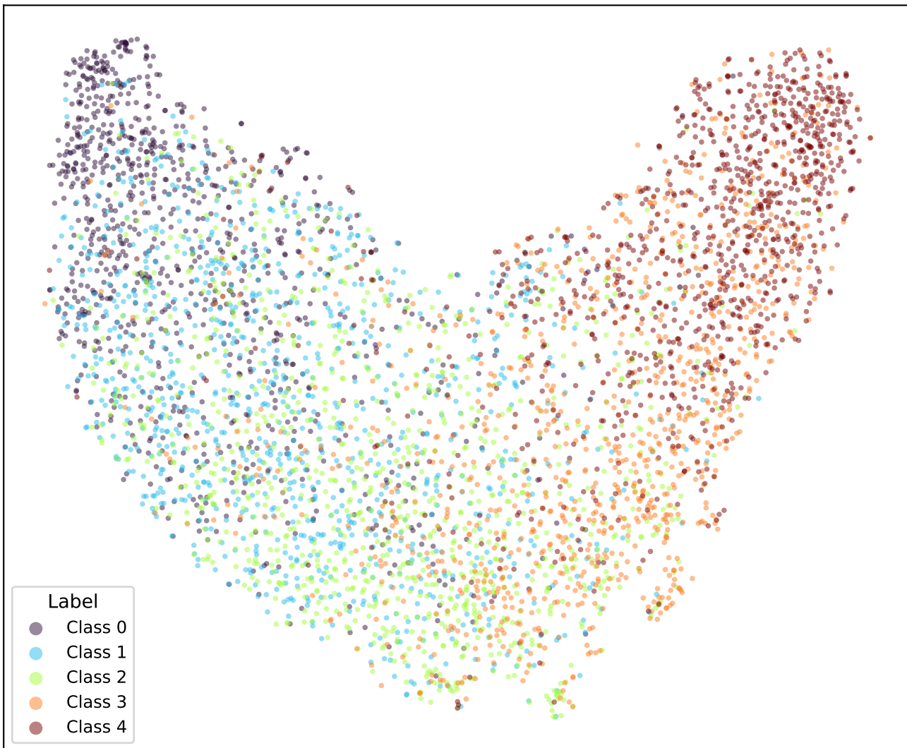
google/bert_uncased_L-2_H-128_A-2-amazon_reviews-SOFT3-TRIPa1-4 (val)
