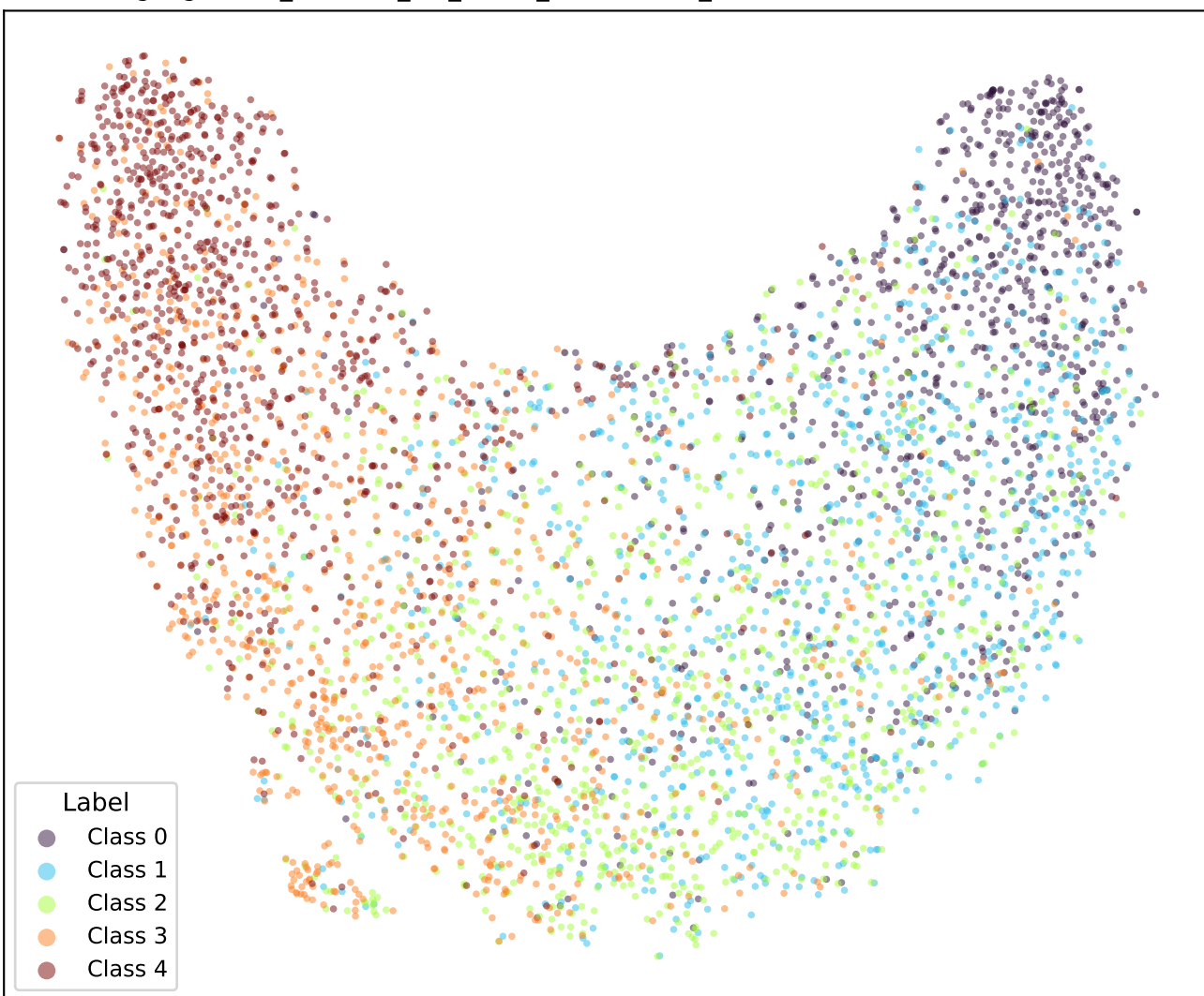
google/bert_uncased_L-2_H-128_A-2-amazon_reviews-SOFT3-TRIPa1-5 (val)
