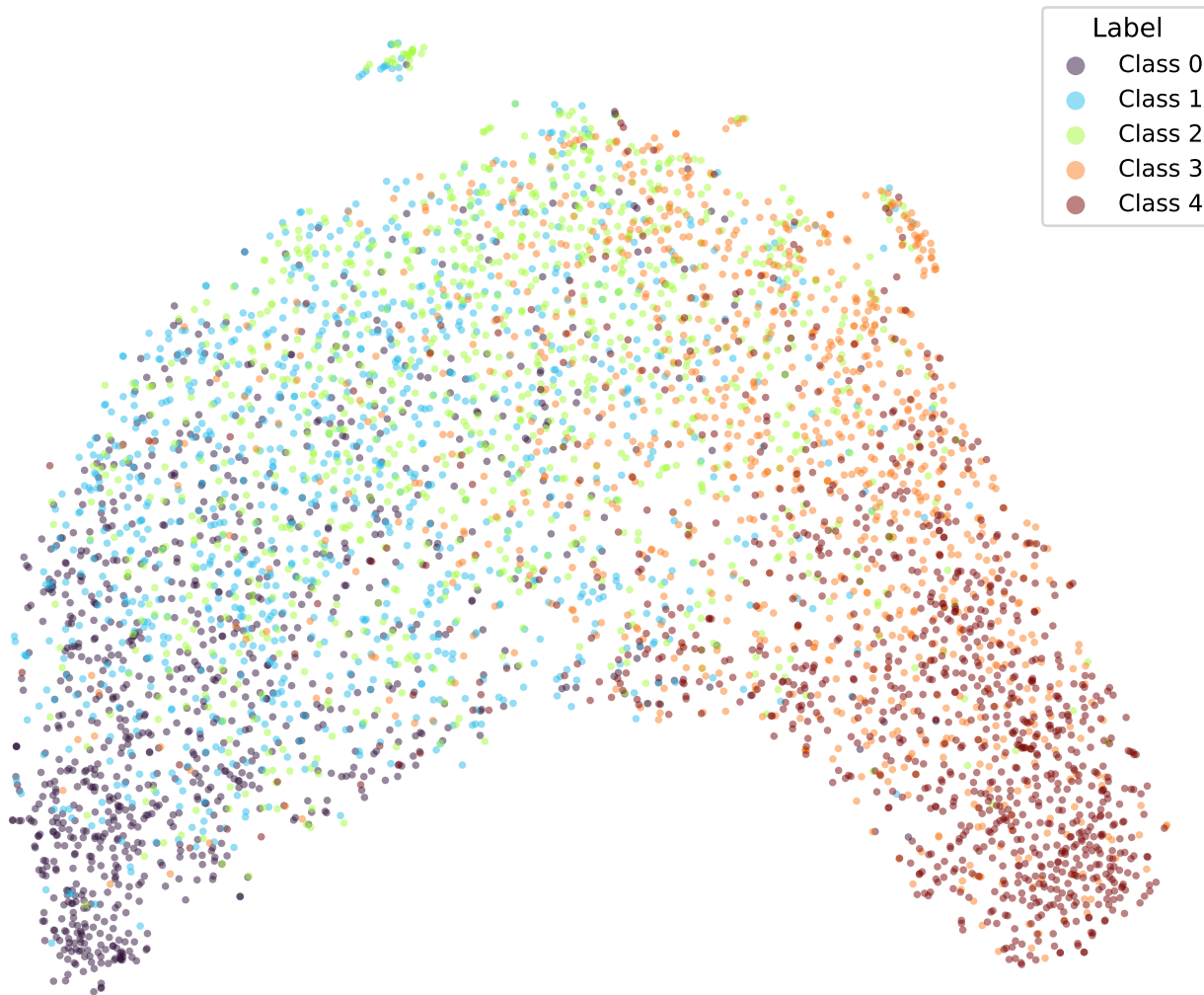
google/bert_uncased_L-2_H-128_A-2-amazon_reviews-SOFT4-TRIPa1-1 (val)
