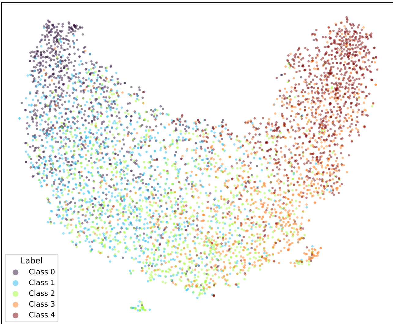
google/bert_uncased_L-2_H-128_A-2-amazon_reviews-SOFT4-TRIPa1-3 (val)
