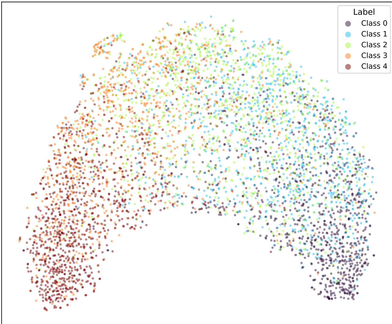
google/bert_uncased_L-2_H-128_A-2-amazon_reviews-SOFT4-TRIPa1-5 (val)
