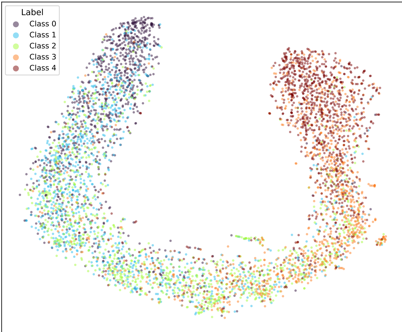
google/bert_uncased_L-2_H-128_A-2-amazon_reviews-WKL-TRIPa1-2 (val)
