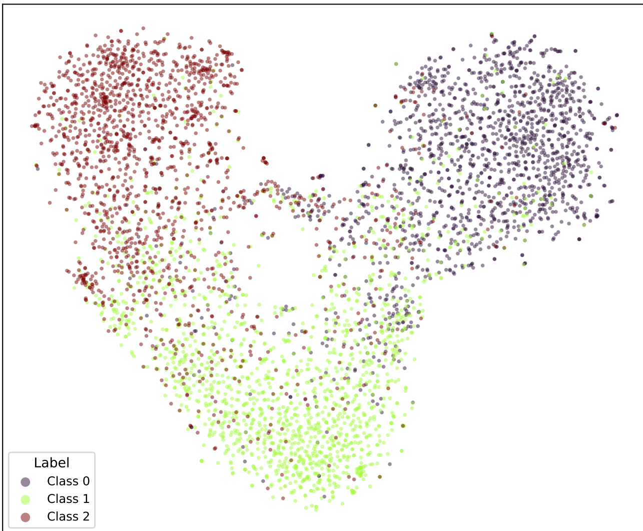
google/bert_uncased_L-2_H-128_A-2-snli-BCE-TRIPa1-1 (val)
