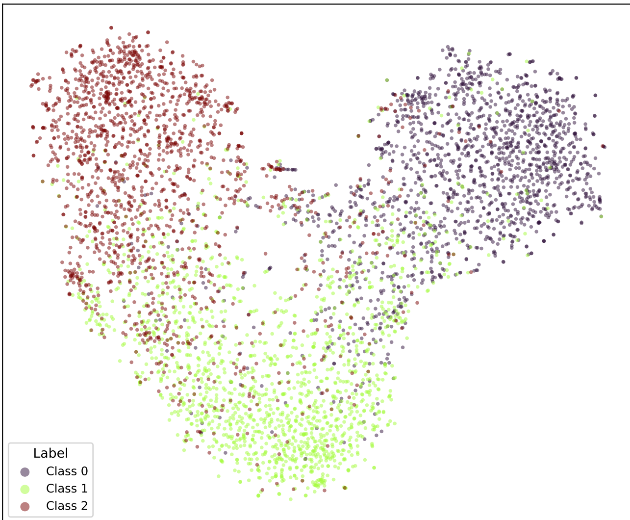
google/bert_uncased_L-2_H-128_A-2-snli-BCE-TRIPa1-4 (val)
