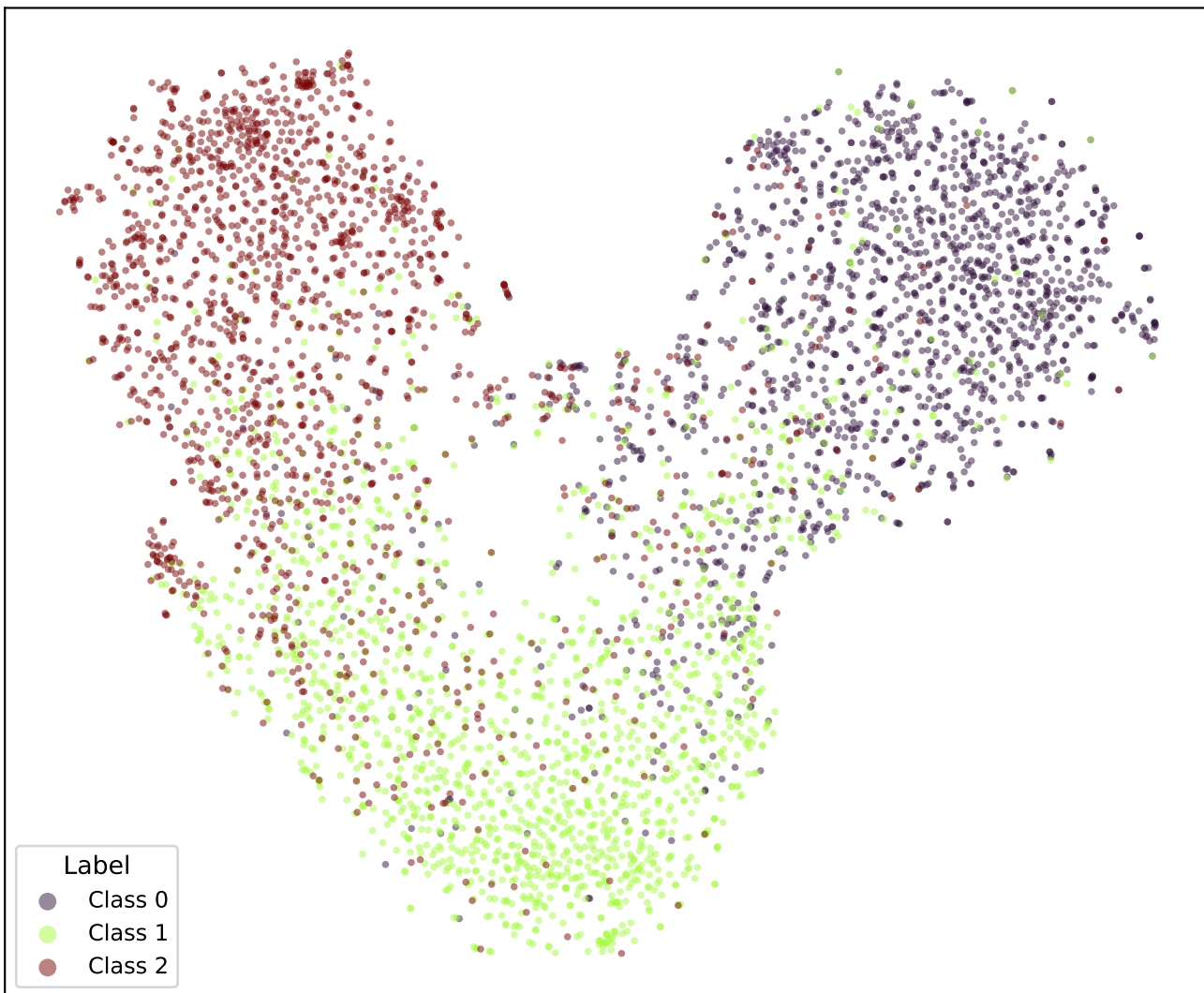
google/bert_uncased_L-2_H-128_A-2-snli-BCE-TRIPa1-5 (val)
