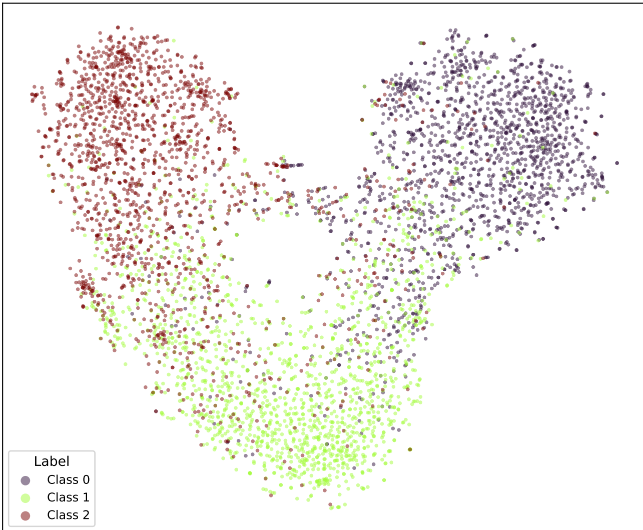
google/bert_uncased_L-2_H-128_A-2-snli-BCE-TRIPa2-4 (val)
