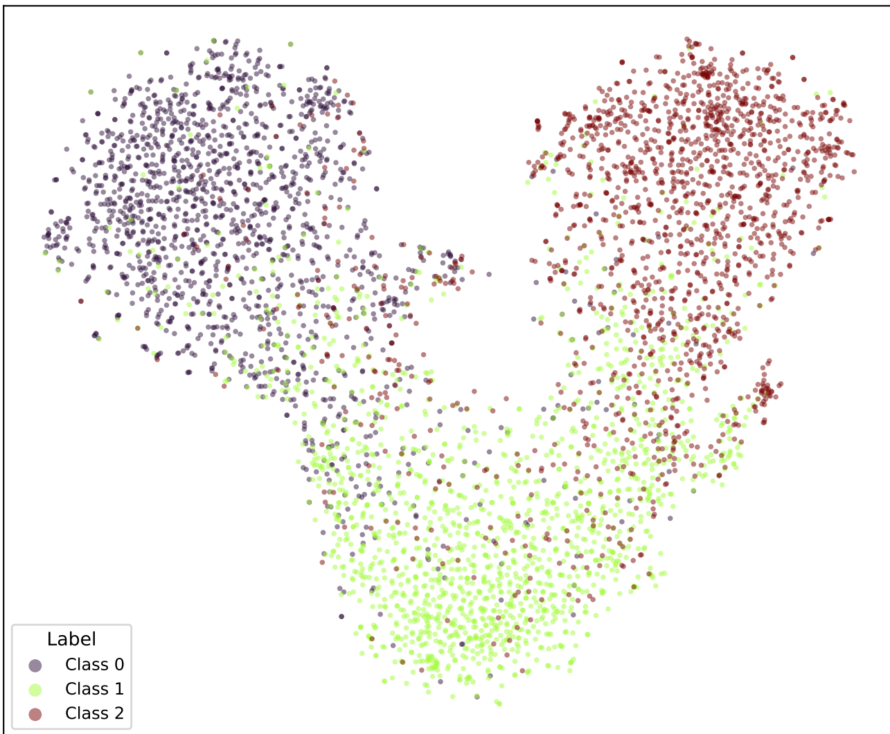
google/bert_uncased_L-2_H-128_A-2-snli-BCE-TRIPa2-5 (val)
