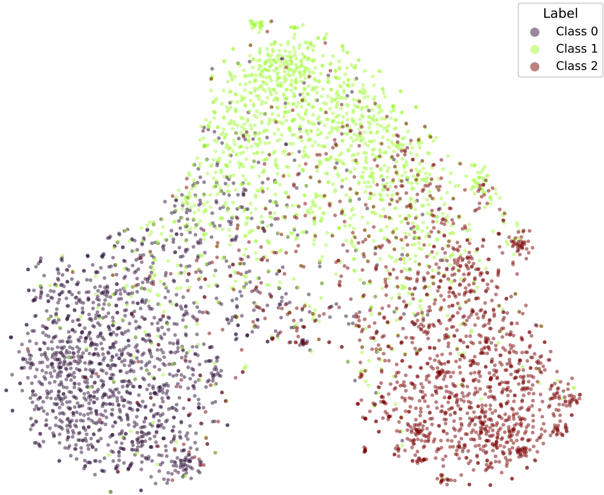
google/bert_uncased_L-2_H-128_A-2-snli-CE-TRIPa1-1 (val)
