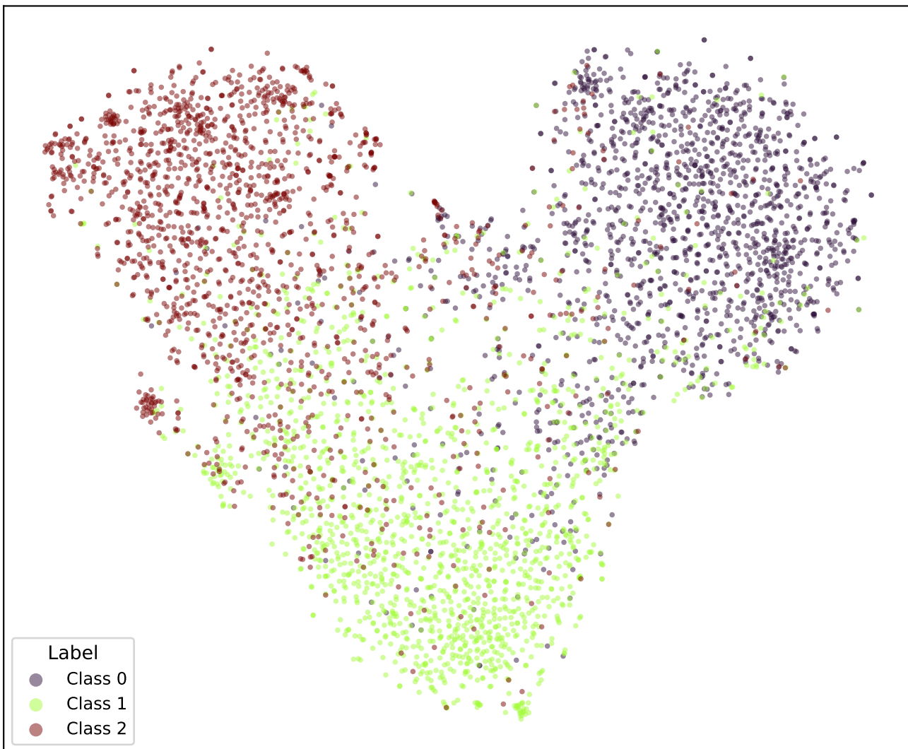
google/bert_uncased_L-2_H-128_A-2-snli-CE-TRIPa1-2 (val)
