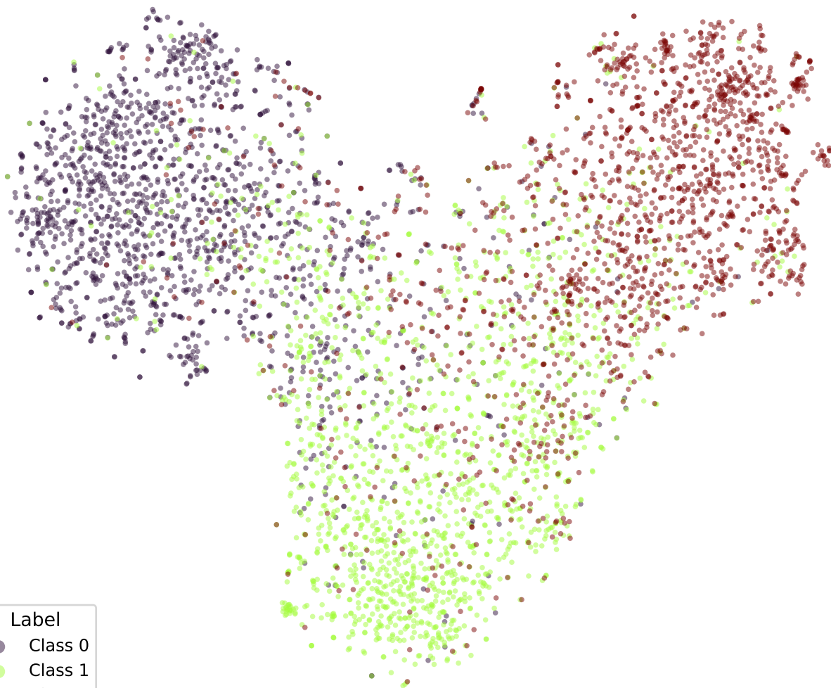
google/bert_uncased_L-2_H-128_A-2-snli-CORAL-TRIPa1-2 (val)
