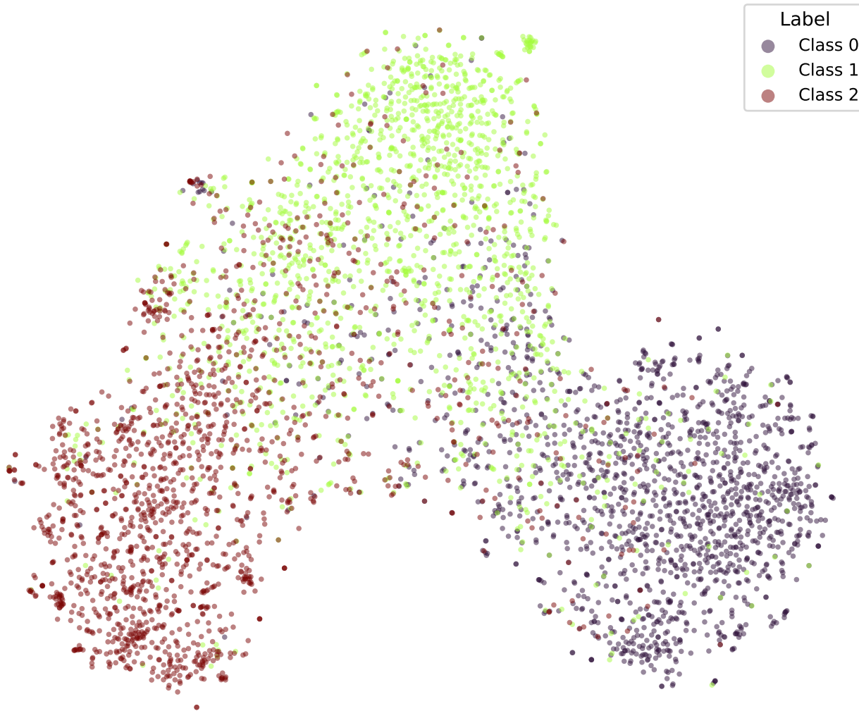
google/bert_uncased_L-2_H-128_A-2-snli-CORAL-TRIPa1-3 (val)
