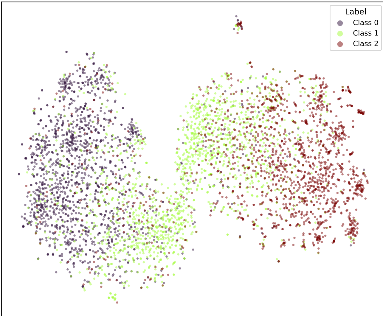
google/bert_uncased_L-2_H-128_A-2-snli-CORAL-TRIPa1-4 (val)
