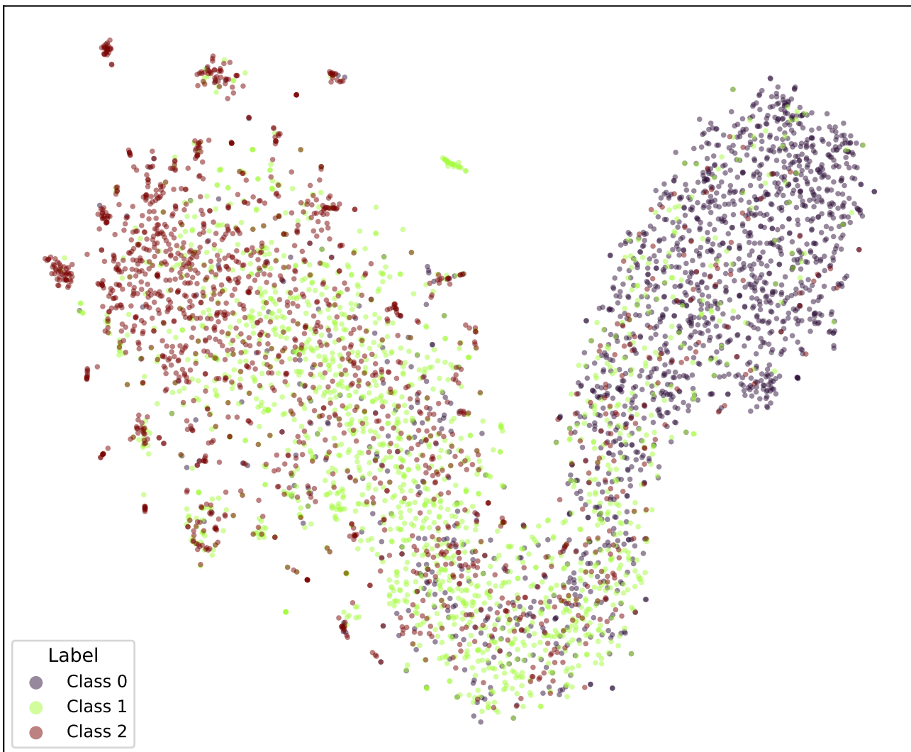
google/bert_uncased_L-2_H-128_A-2-snli-CORAL-TRIPa2-2 (val)
