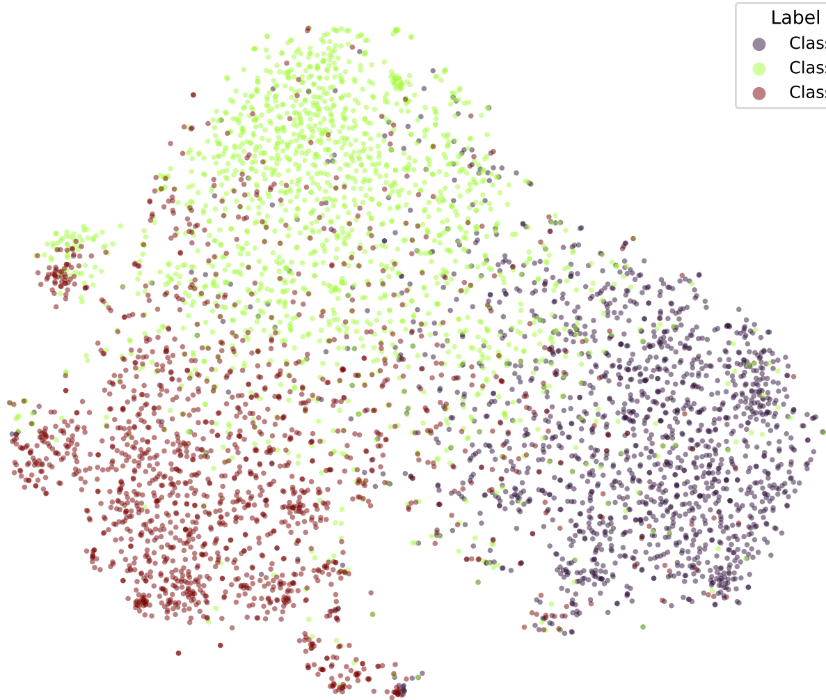
google/bert_uncased_L-2_H-128_A-2-snli-CORN-1 (val)
