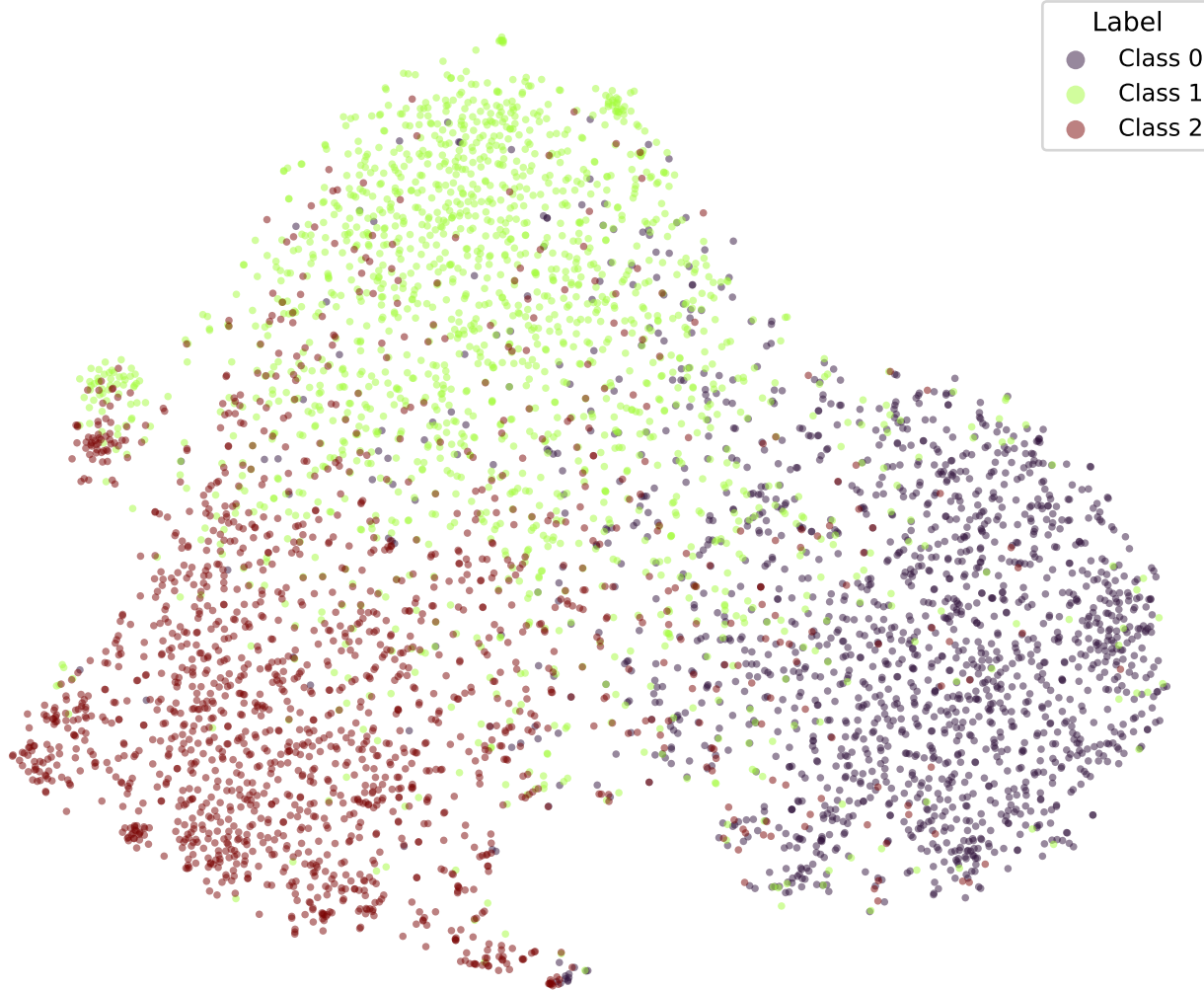
google/bert_uncased_L-2_H-128_A-2-snli-CORN-3 (val)
