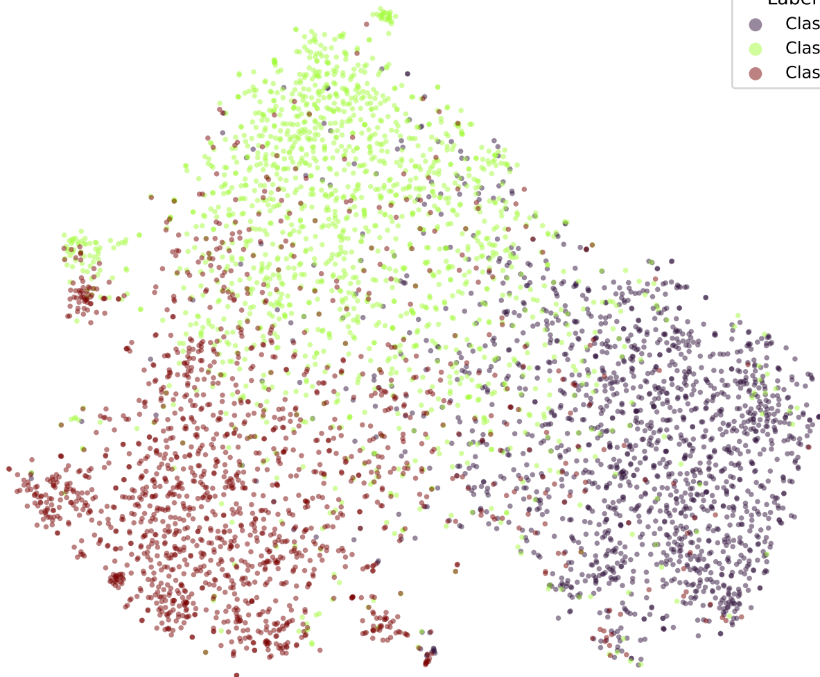
google/bert_uncased_L-2_H-128_A-2-snli-CORN-5 (val)
