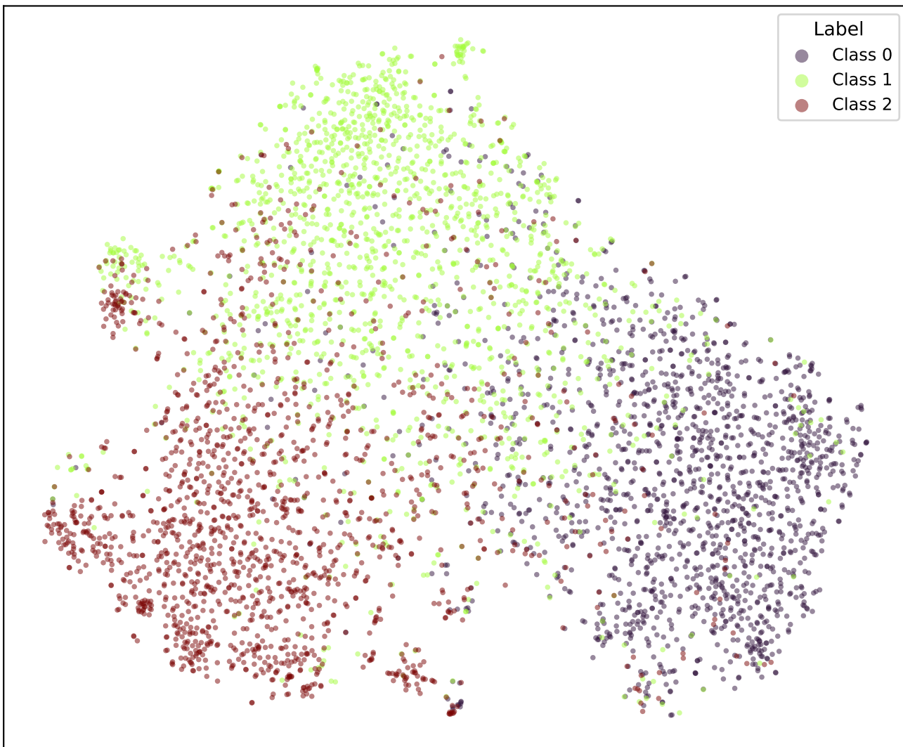
google/bert_uncased_L-2_H-128_A-2-snli-CORN-5 (val)
