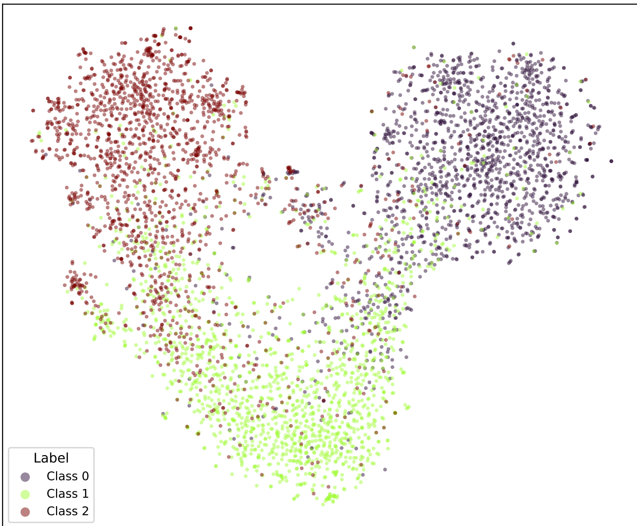
google/bert_uncased_L-2_H-128_A-2-snli-EMD-TRIPa1-2 (val)
