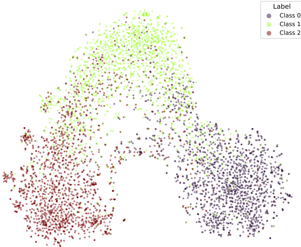
google/bert_uncased_L-2_H-128_A-2-snli-EMD-TRIPa2-1 (val)
