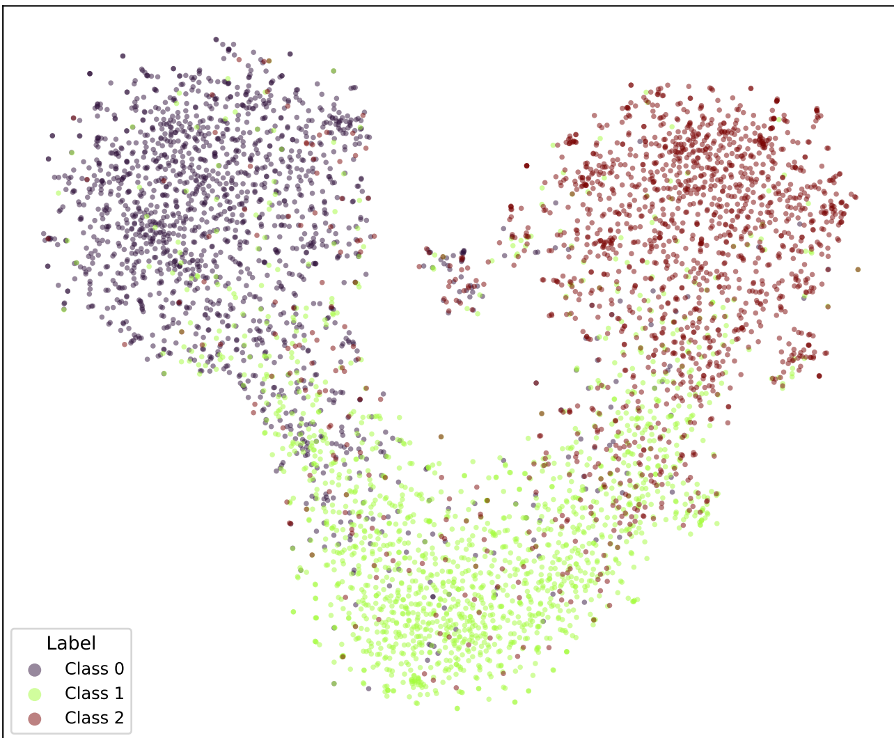
google/bert_uncased_L-2_H-128_A-2-snli-EMD-TRIPa2-2 (val)
