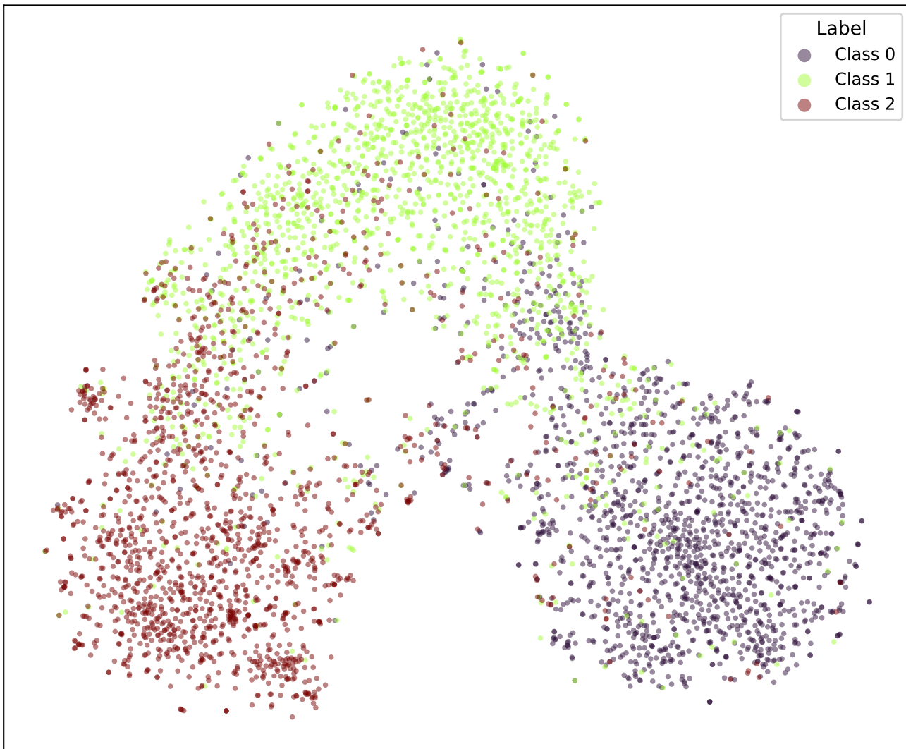
google/bert_uncased_L-2_H-128_A-2-snli-EMD-TRIPa2-5 (val)
