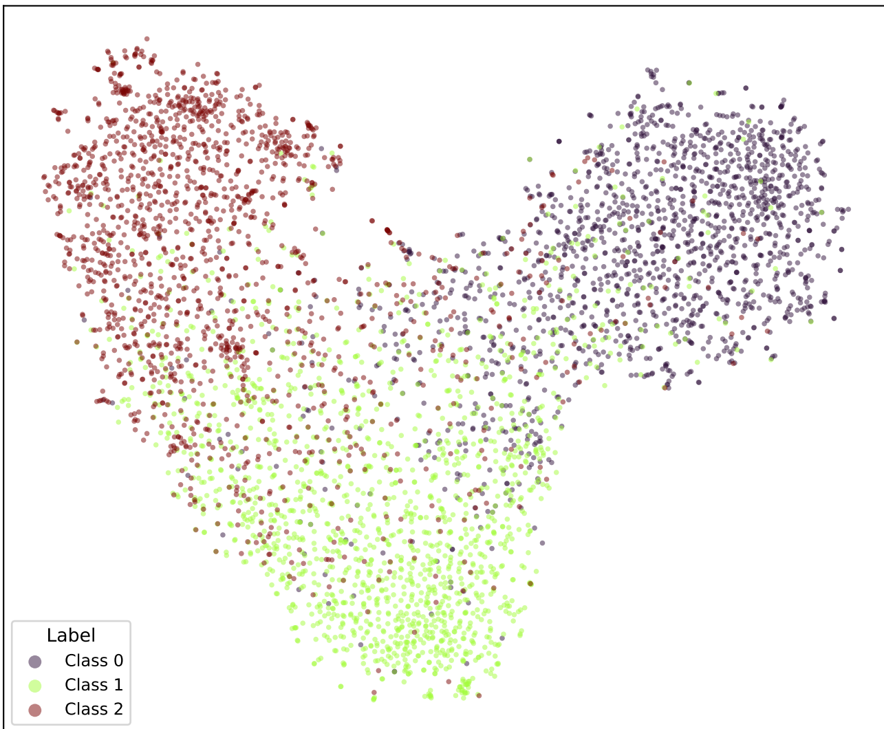
google/bert_uncased_L-2_H-128_A-2-snli-OLL1-TRIPa1-5 (val)
