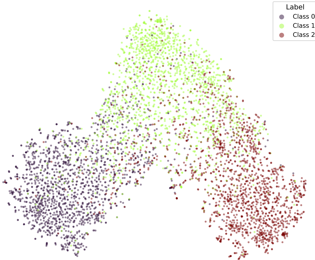
google/bert_uncased_L-2_H-128_A-2-snli-OLL15-TRIPa1-3 (val)
