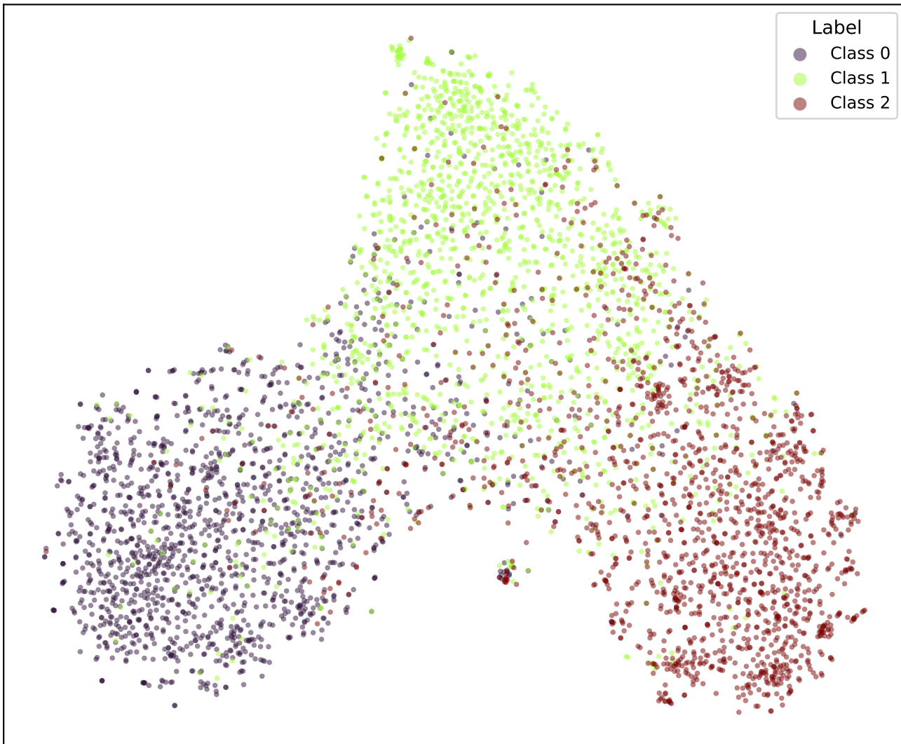
google/bert_uncased_L-2_H-128_A-2-snli-OLL2-TRIPa1-2 (val)
