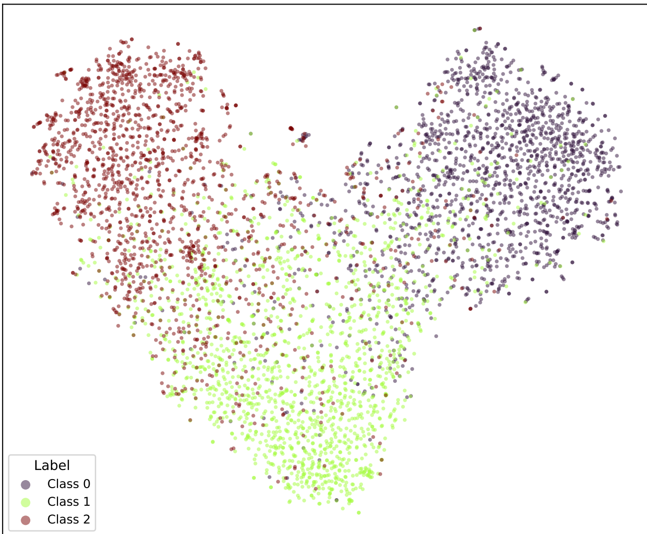
google/bert_uncased_L-2_H-128_A-2-snli-OLL2-TRIPa1-4 (val)
