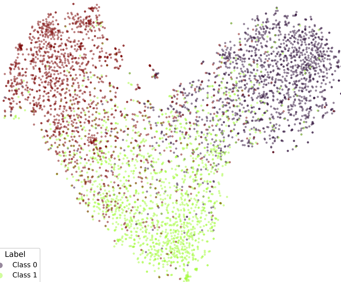
google/bert_uncased_L-2_H-128_A-2-snli-OLL2-TRIPa1-5 (val)
