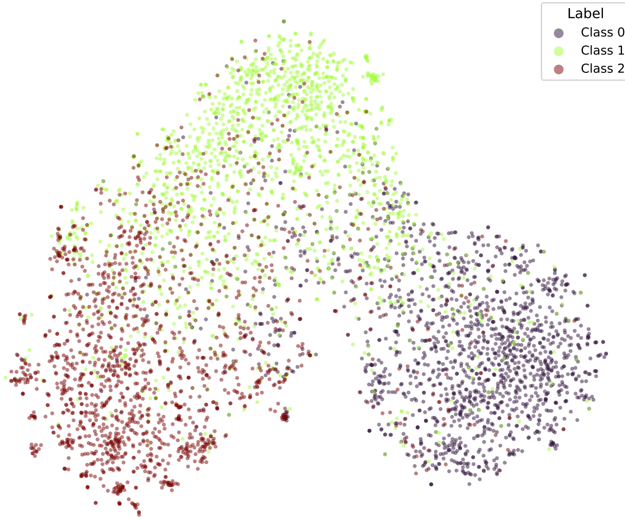
google/bert_uncased_L-2_H-128_A-2-snli-SOFT2-TRIPa1-4 (val)
