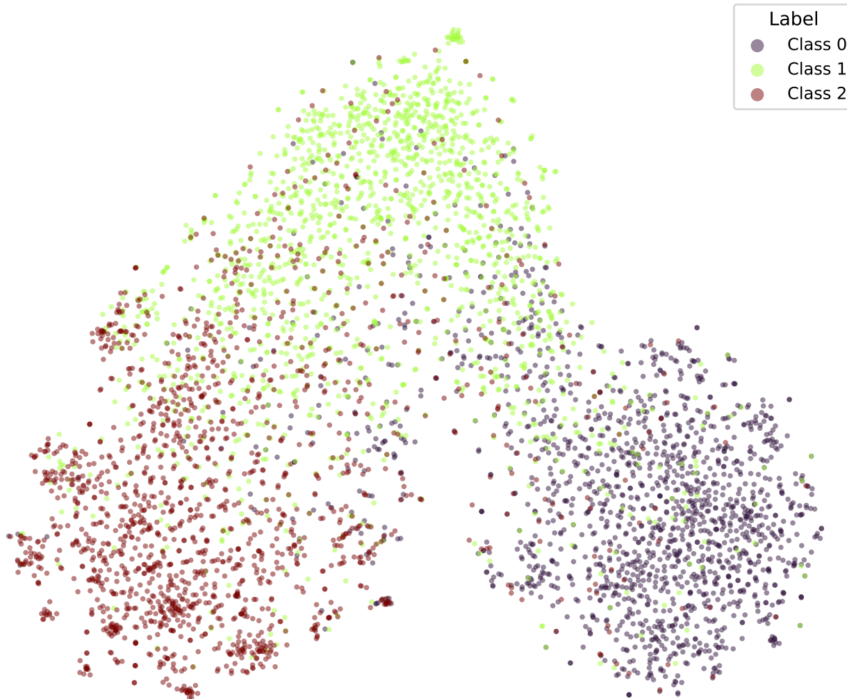
google/bert_uncased_L-2_H-128_A-2-snli-SOFT2-TRIPa2-1 (val)
