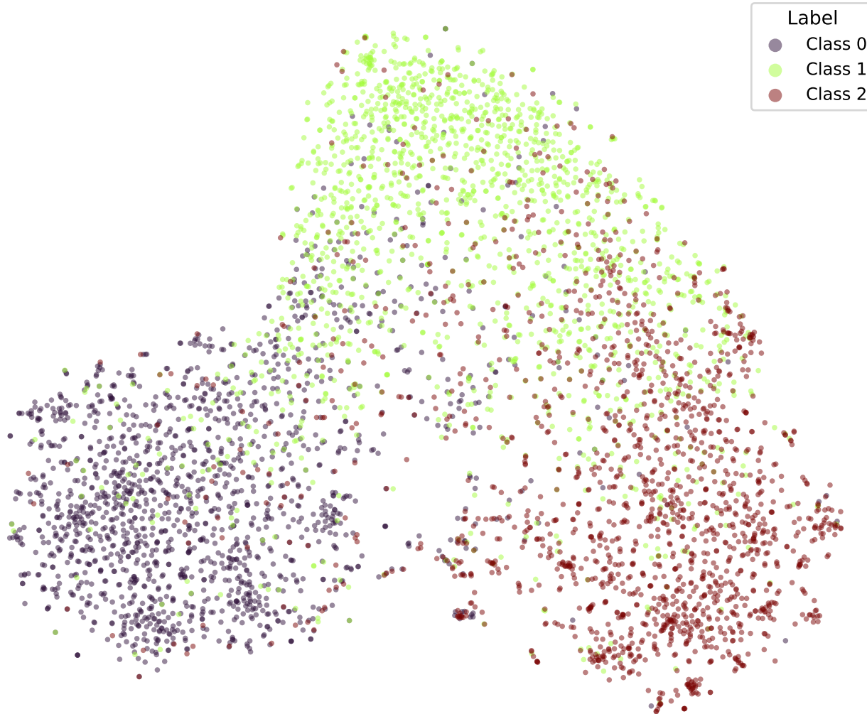
google/bert_uncased_L-2_H-128_A-2-snli-SOFT2-TRIPa2-3 (val)
