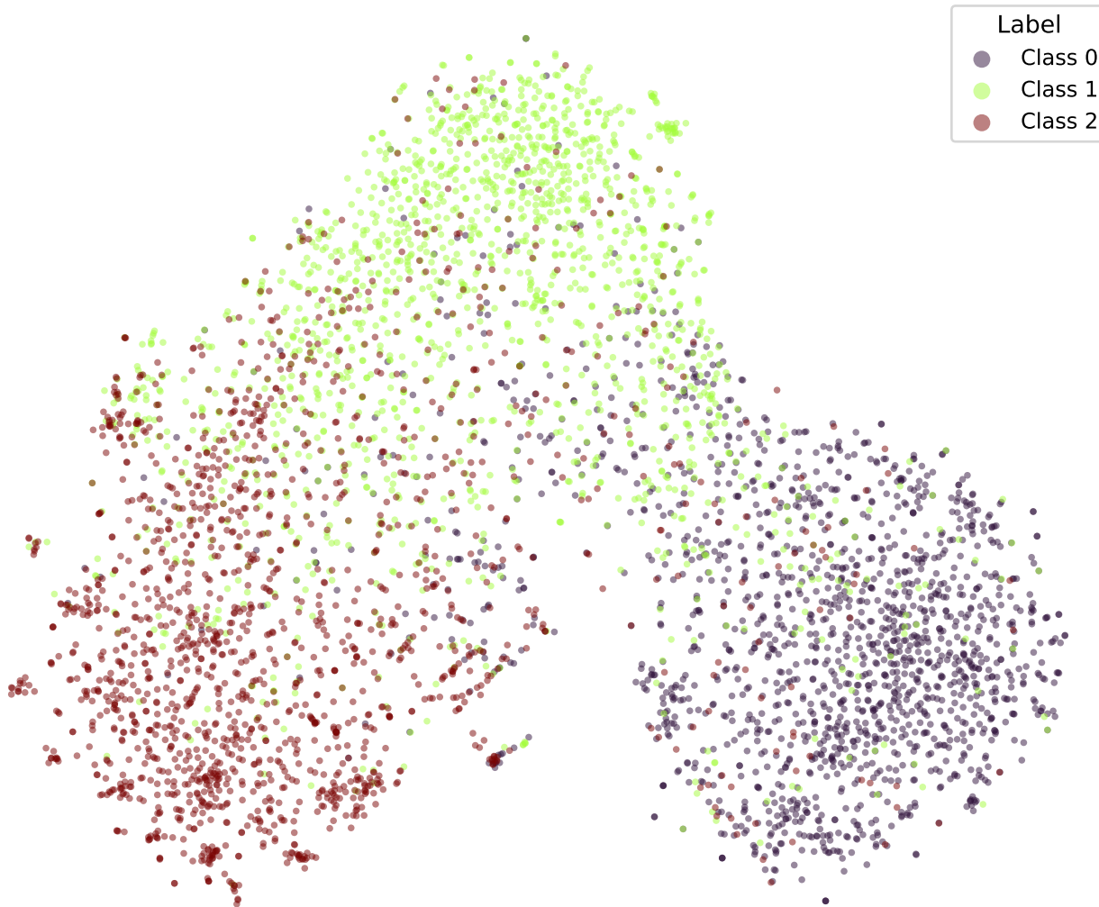
google/bert_uncased_L-2_H-128_A-2-snli-SOFT2-TRIPa2-4 (val)
