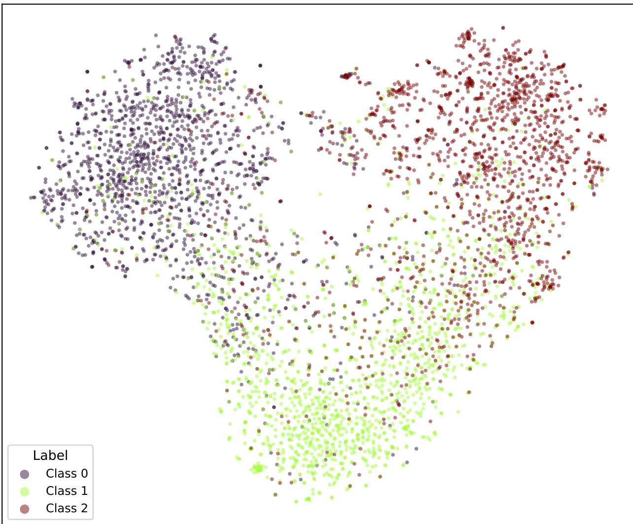
google/bert_uncased_L-2_H-128_A-2-snli-SOFT2-TRIPa2-5 (val)
